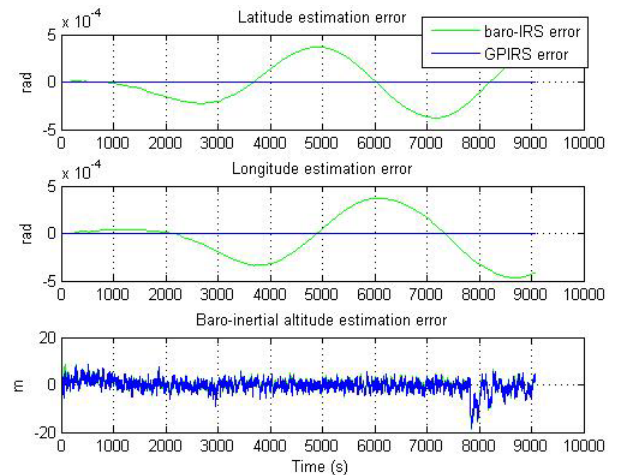
Fig. 9. IRS and GPIRS position estimation errors
