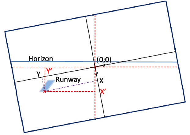
Fig. 4. Impact of roll angle on video measurements
