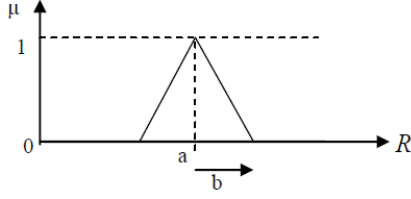
Figure 3: Example of dual representation of a fuzzy number
