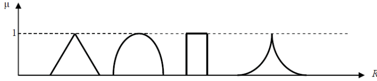
Figure 4: Examples of shapes for fuzzy dual numbers
