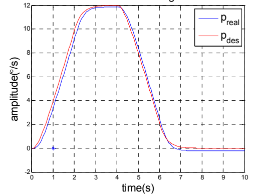
(a) Result of interior point real and desired roll angular rate
