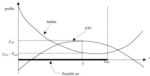
Figure 10 - Solution of the private ATC/ATM supplier problem (no real roots for (85)).
