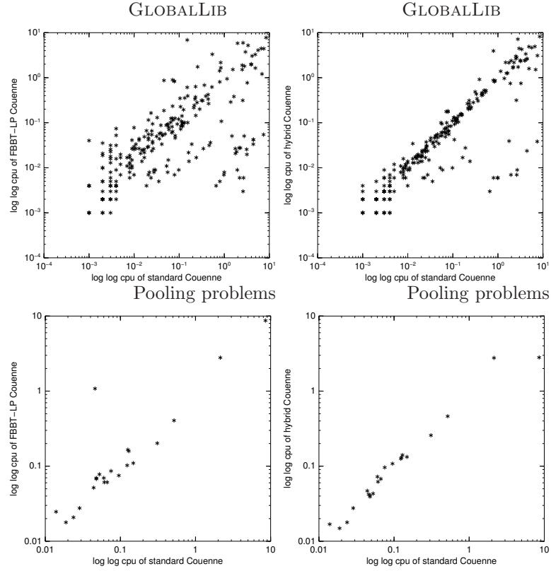
Figure 2: User CPU time scatter plots of FBFT-LPC (left) and hybrid (right) versus standard COUENNE versions on continuous NLP instances from GLOBALLIB (top) and the pooling problems (bottom).
