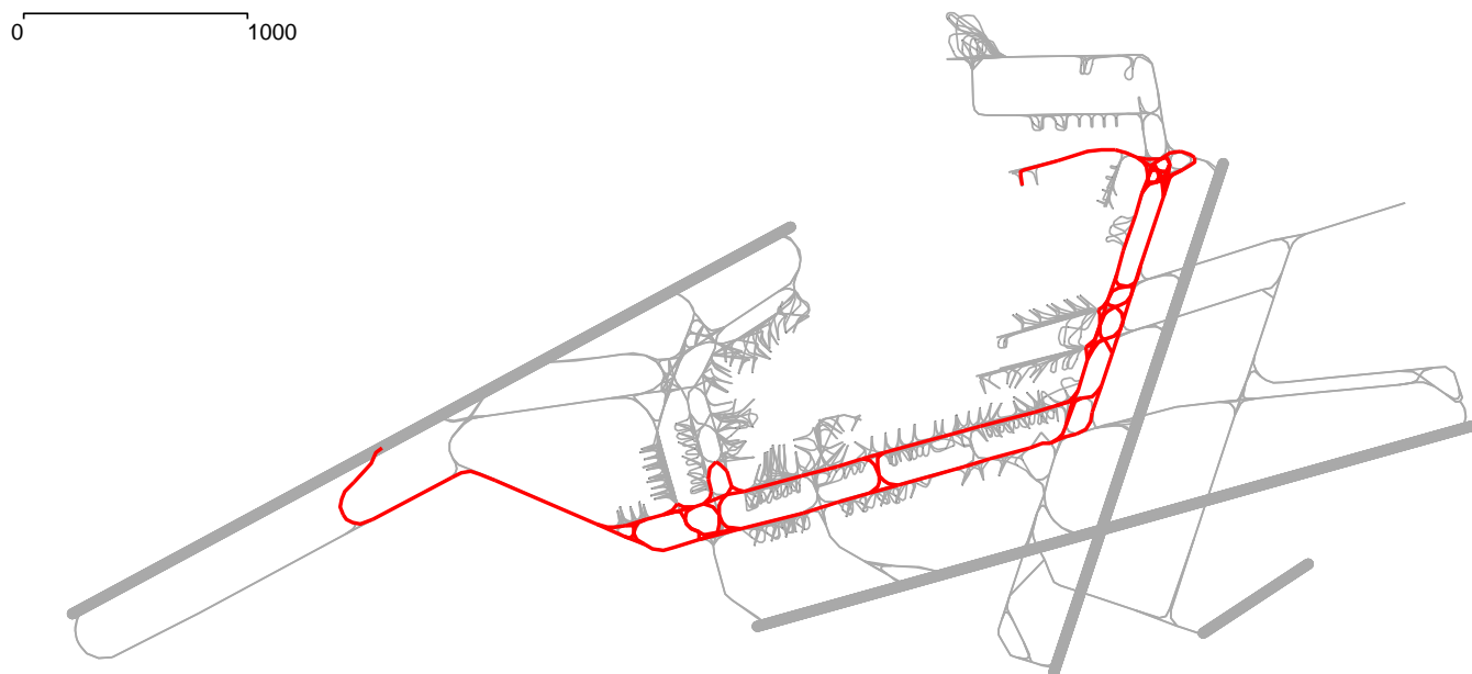
Figure 1: Roissy airport graph - Example of shortest and alternate paths
