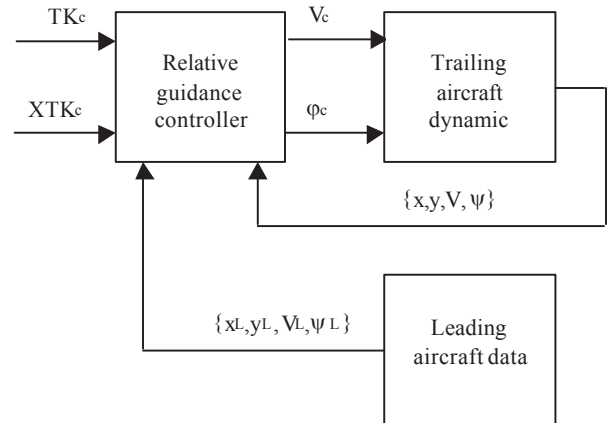
Figure 2 Block diagram of the relative guidance control system
