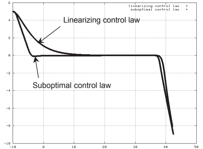
Figure 7 Movement of the trailing aircraft in the horizontal plane (axes in NM)
