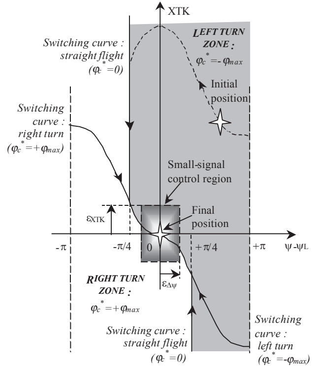
Figure 5 Modified 'cross track' suboptimal control law
