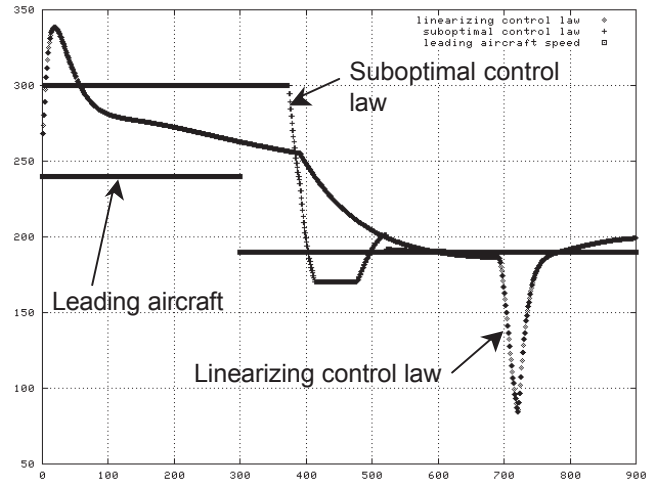
Figure 11 Commanded speed (in kts) as a function of time (in sec)
