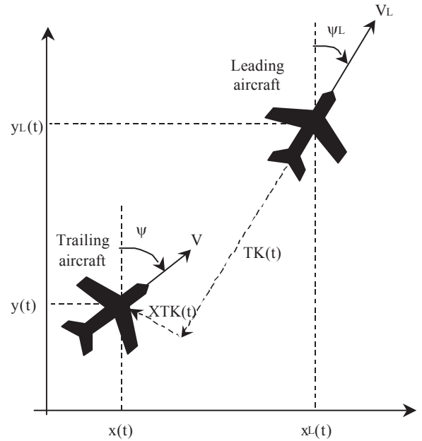
Figure 1 Reference frame affixed to the leading aircraft
