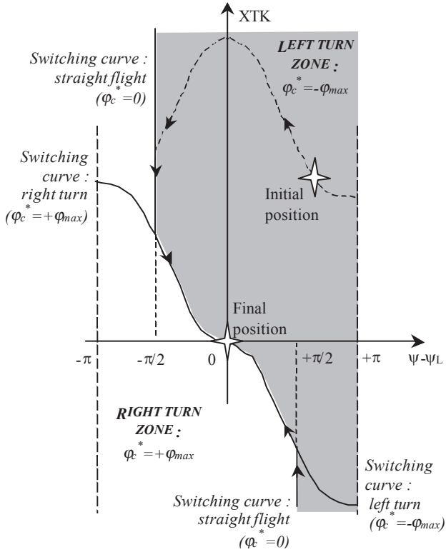
Figure 4 'cross track' suboptimal control law
