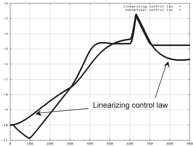
Figure 9 'Along track' distance (TK, in NM) between the leading and the trailing aircraft as a function of time (in sec)
