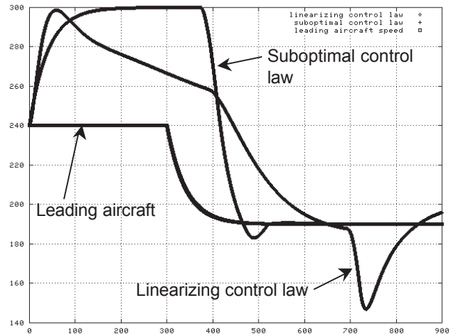
Figure 12 Actual speed (in kts) as a function of time (in sec)
