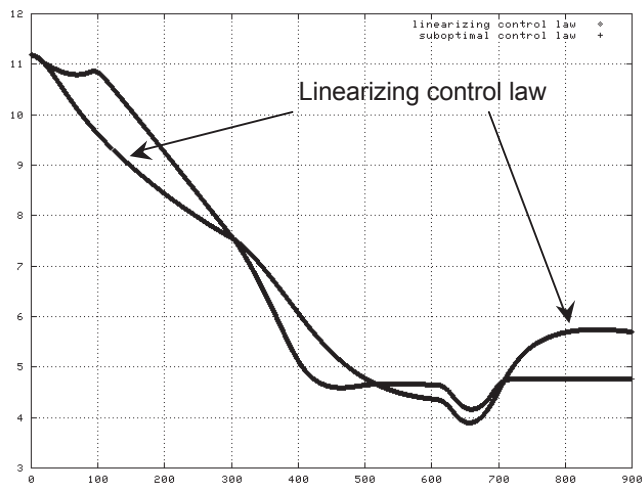
Figure 10 Slant range (in NM) between the leading and the trailing aircraft as a function of time (in sec)
