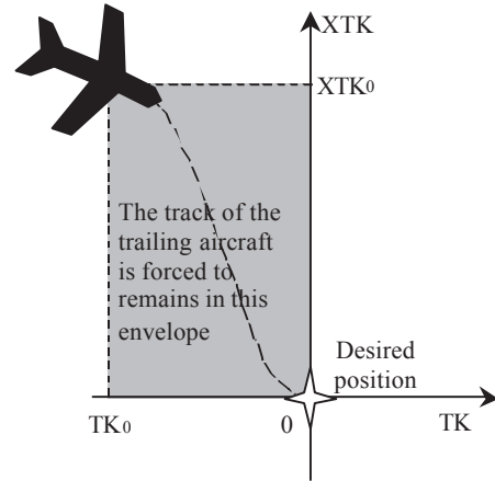
Figure 3 Track envelope of the trailing aircraft
