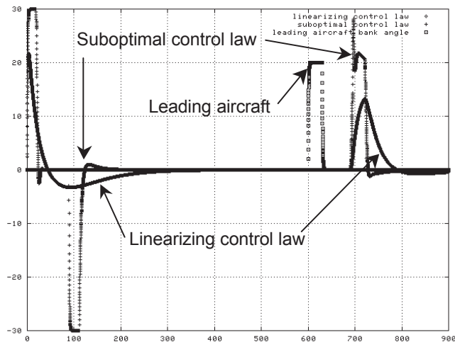
Figure 14 Actual bank angle (in degrees) as a function of time (in sec)
