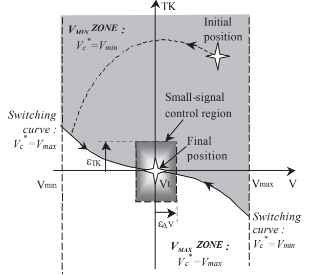
Figure 6 'along track' suboptimal control law
