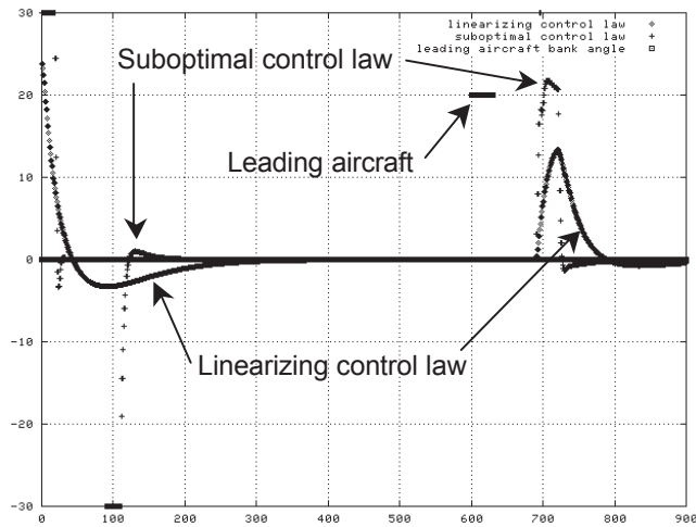
Figure 13 Commanded bank angle (in degrees) as a function of time (in sec)
