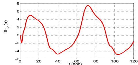
Fig.8(c) Lateral tracking error with correction
