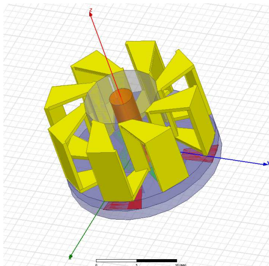
Figure 5: Antenna structure
