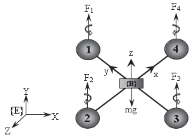
Fig. 1. Quadrotor Configuration
