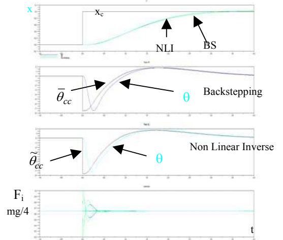
Fig.3. Step response of \phi ( \omega_\phi=15 rad/s)
