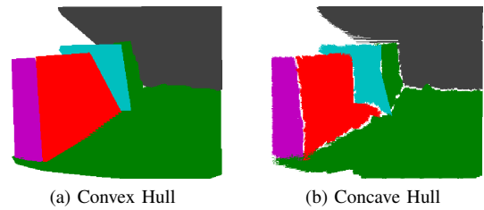
Fig. 10: Polygonization results
