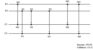
Figure 12: Marker exchange between parents. The parents are labeled P_1 and P_2 , the children C_1 and C_2 . First the marker of both parent are gathered together and ordered according their layer level. Then, the first child C_1 take one maker over two in the ordered list, and the child C_2 takes the remaining ones.
