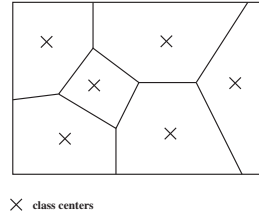
Figure 3: Random sectoring by Voronoi diagram.
