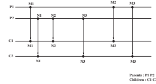
Figure 12: Marker exchange between parents. The parents are labeled P_1 and P_2 , the children C_1 and C_2 . First the marker of both parents are gathered together and ordered according to their layer level. Then, the first child C_1 takes one marker over two in the ordered list, and the child C_2 takes the remaining ones.
