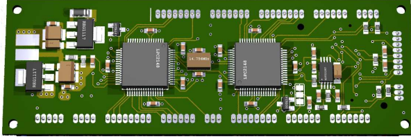
Figure 4: The dual processor classic controller board
