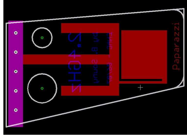
Figure 14: Custom 8cm airborne antenna (2.4GHz) designed to be included in the fin of an aircraft.
