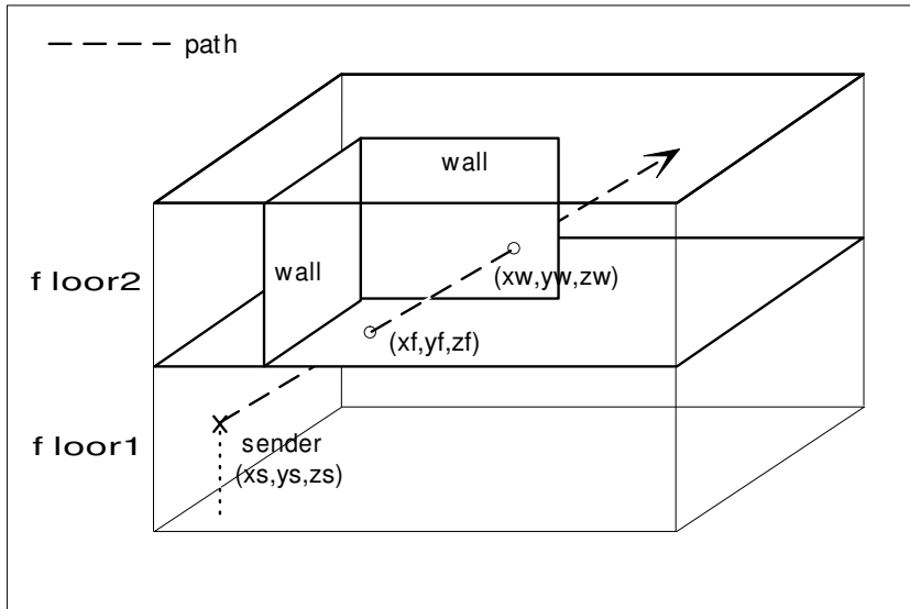
Figure 4: Path from transmitter intersecting a ceiling and a wall
