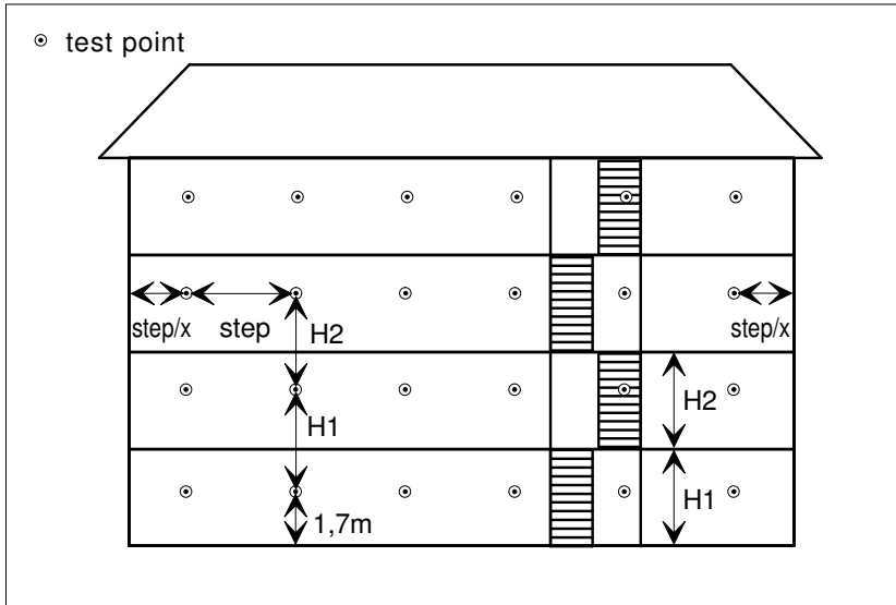
Figure 3: Grid of test points in a building
