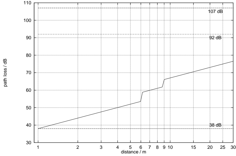
Figure 2: Path loss with additional attenuation at 6m and 9m due to walls
