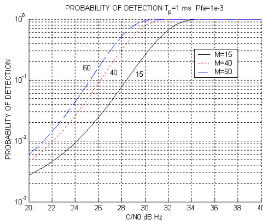
Figure 6: Probability of detection versus total (I+Q) C/N_0 at the antenna output using the I and Q components for 1 ms coherent integration time with the first approach and without front end filtering effects
