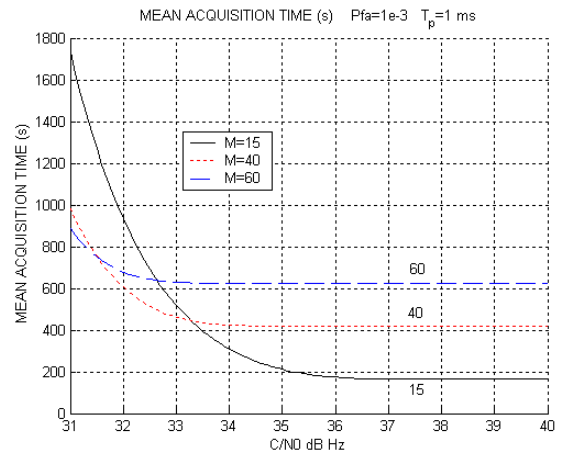
Figure 4: Single dwell search mean acquisition time versus total (I+Q) C/N 0 at antenna output using only one component I or Q for P_{fa} = 1e-3 , 1 ms coherent integration time and when searching only one doppler bin and without front end filtering effects
