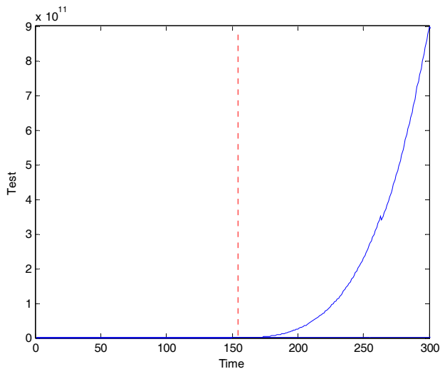
Figures 5 & 6: Adapted sequential constrained GLR test: injection of combined step-ramp pseudo-range bias The studied algorithm performs better here since it detects this type of error quite instantaneously (figure 6).
