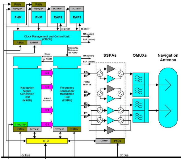
Figure 1: Galileo generic payload
