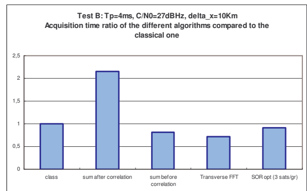
Figure 9: Acquisition time ratio of the different algorithms compared to the classical one for a signal of 27dBHz , with fixed T_p
