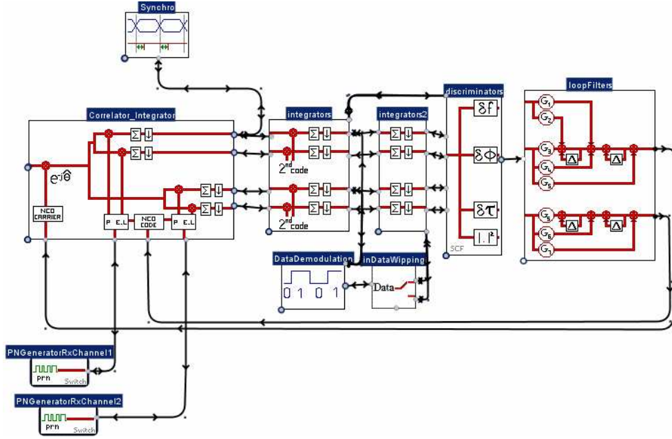
Fig. 3: Tracking architecture
