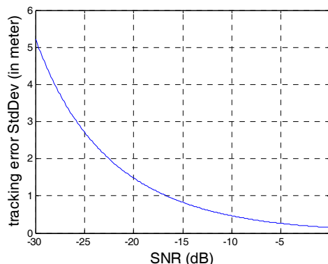
Figure 5: Tracking error standard deviation versus SNR
