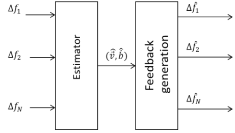
Figure 11 VPLL implementation
