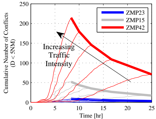
Fig. 6: Cumulative number of potential conflicts for 1-3X traffic intensity.
