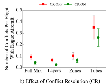
Figure 14: Number of conflicts per flight with rogue aircraft
