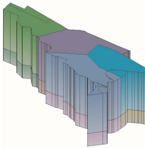
495 Fig. 13 Eight elementary sectors of the Maastricht ACC (EDYYBUTA).
