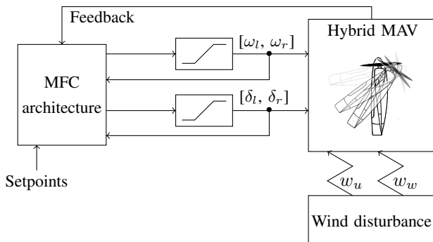
Fig. 7: MFC architecture designed for HMAVs with saturated control inputs. Propeller speeds ( \omega_l, \omega_r ) and flap deflections ( \delta_l, \delta_r ) are computed by means of MFC architecture block.
