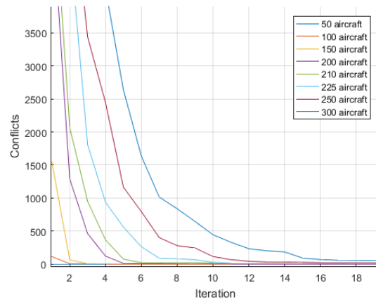
Fig. 9. Number of conflicts evolution with respect to iterations
