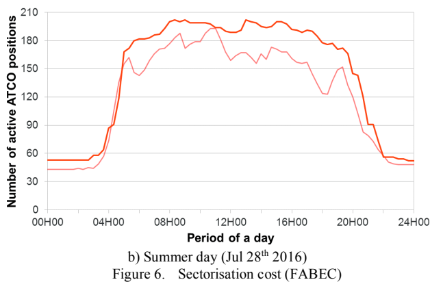
Figure 6. Sectorisation cost (FABEC)
