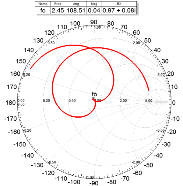
Fig. 4 Simulated Smith chart of the proposed ARDRA.
