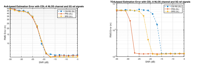
Figure 2. Root Mean Square positioning Errors (RMSE) for CSI-RS, SRS, and PRS signals in a CDL NLOS channel. Left: AoA estimator; right: ToA estimator.
